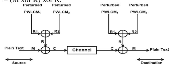
Fig 2. RFCA Scheme
