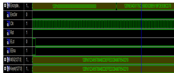
Fig 5. Encryption Algorithm
