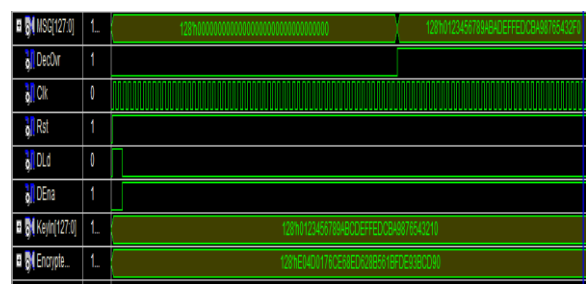
Fig 6. Decryption Algorithm
